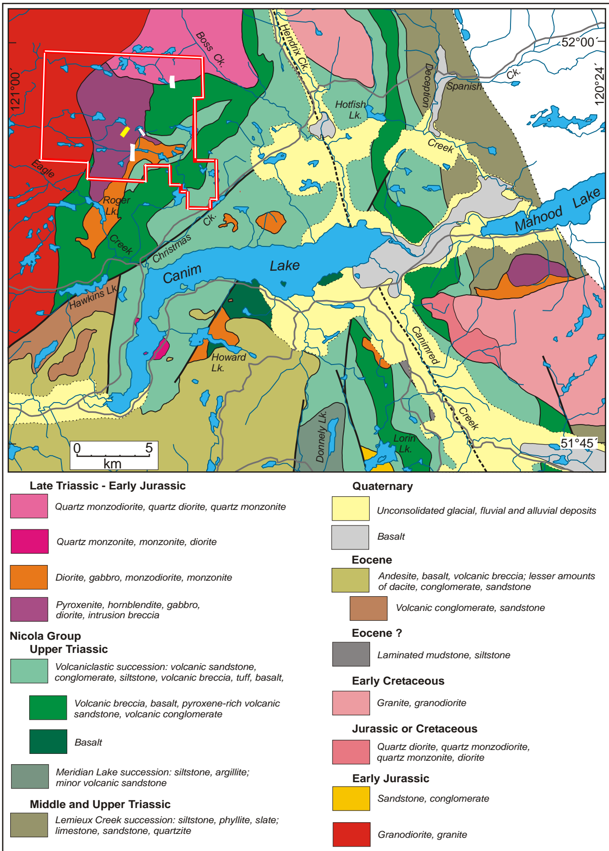
Figure Generalized geology of the Canim Lake map area, based mainly on 2005 fieldwork.
